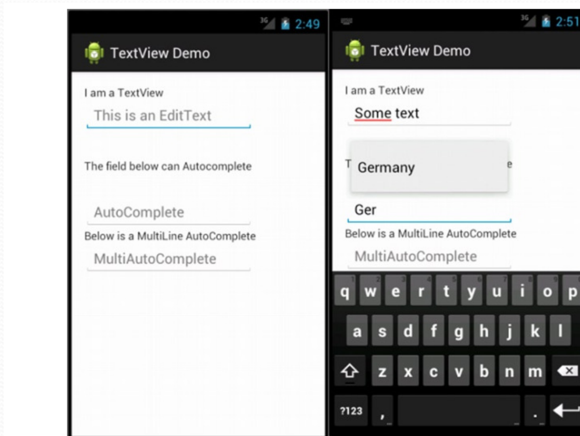
Figure 3-2. Text controls in Android
