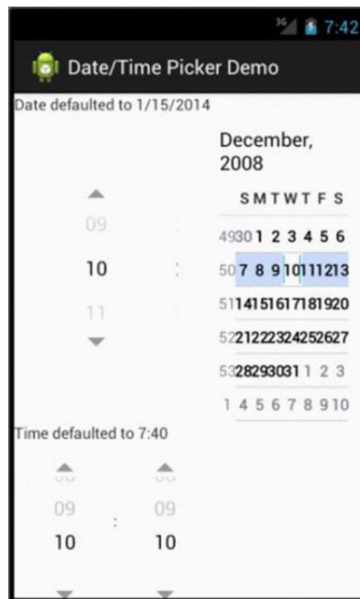
Figure 3-7. The DatePicker and TimePicker UIs
